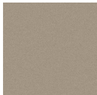
Champán
